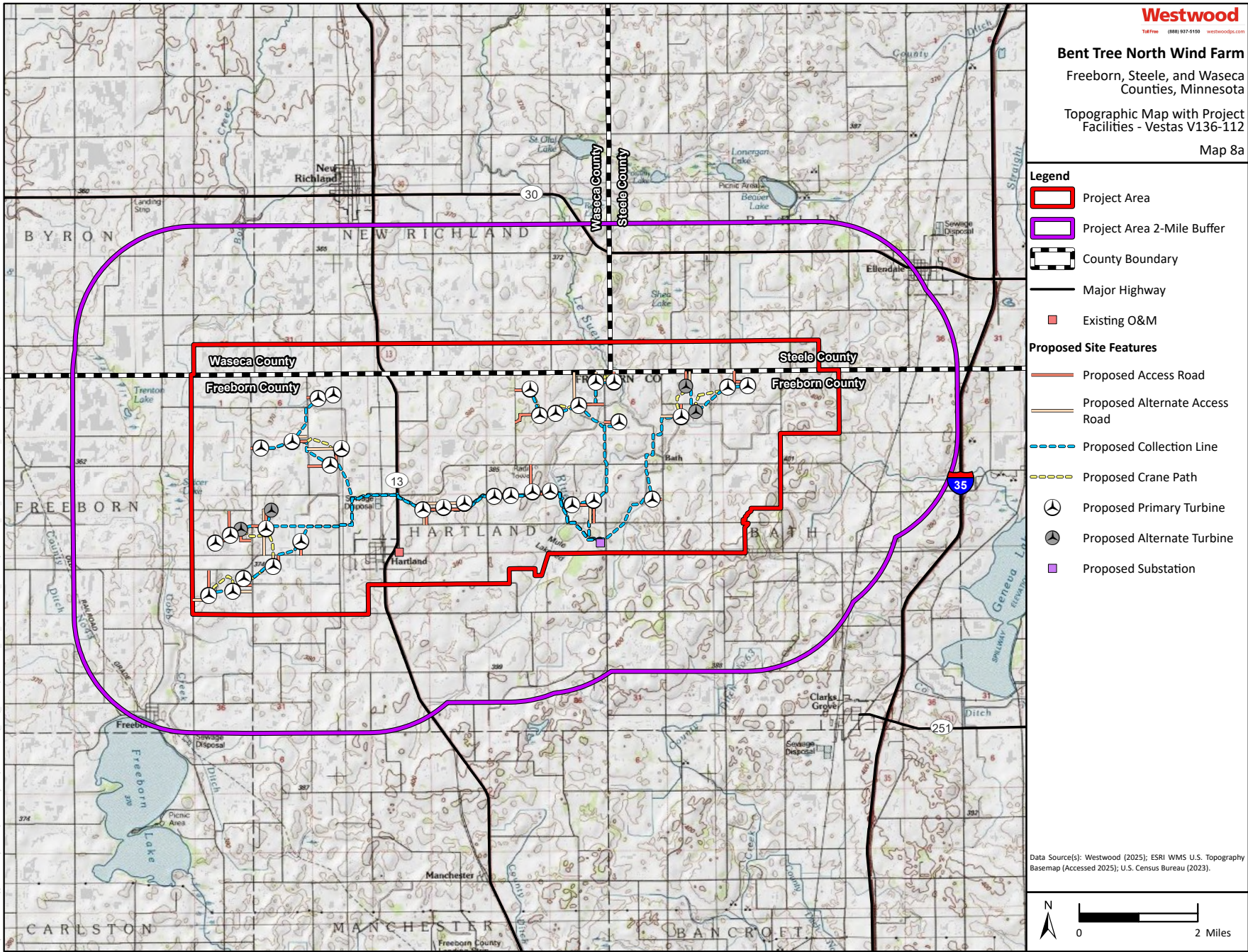
Map 8a: Topographic Map with Project Facilities - Vestas V136 - 112
