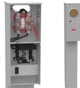
Pictured: U6221-O-200-10GR
